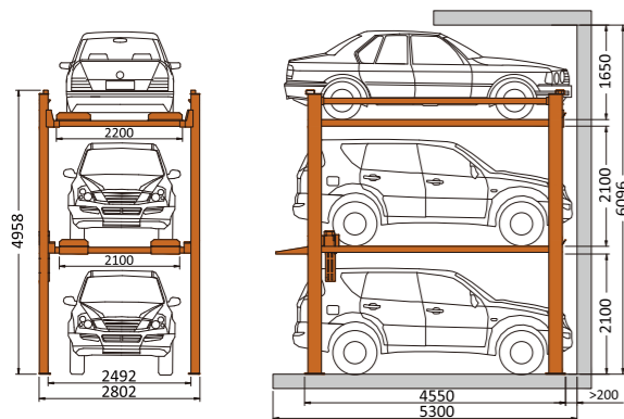
Hydro-Park 2525
