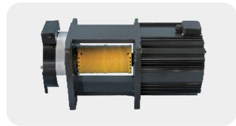
NexusHome Grip ® Strong Drive Traction Motor 强驱式别墅电梯
