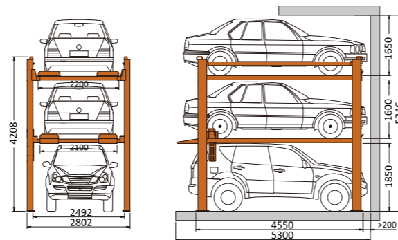
Hydro-Park 2625
